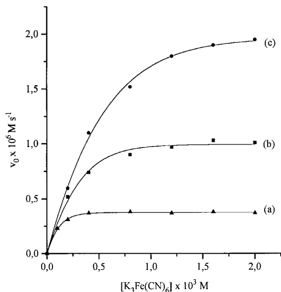
Figure 1. Dependence of v_0 on [\text{K}_3\text{Fe}(\text{CN})_6] . [\text{Ru}(\text{VI})] = 4 \times 10^{-6} \text{ M} , I = 0.5 \text{ M} and T = 30^\circ\text{C} ; (a) [\text{NaOH}] = 0.3 \text{ M} , [\text{2-propanol}] = 0.2 \text{ M} ; (b) [\text{NaOH}] = 0.2 \text{ M} , [\text{2-propanol}] = 0.4 \text{ M} ; (c) [\text{NaOH}] = 0.1 \text{ M} , [\text{2-propanol}] = 0.5 \text{ M}
