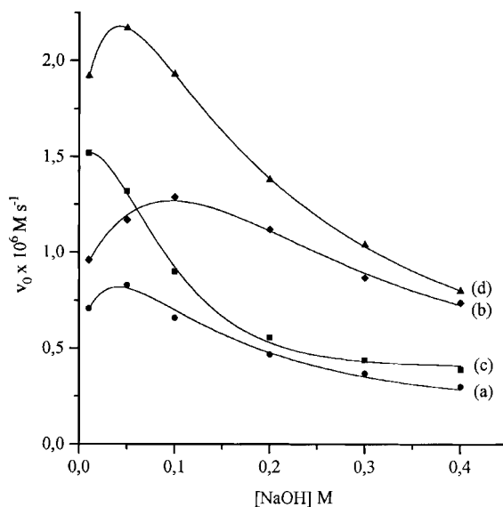
Figure 3. Variation of v_0 with respect to [NaOH]. [Ru(VI)] = 4 \times 10^{-6} M , I = 0.5 M and T = 30^\circ C [K_3Fe(CN)_6] = 0.4 \times 10^{-3} M : (a) [2-propanol] = 0.2 M; (b) [2-propanol] = 0.6 M. [K_3Fe(CN)_6] = 1.2 \times 10^{-3} M : (c) [2-propanol] = 0.2 M; (d) [2-propanol] = 0.6 M
