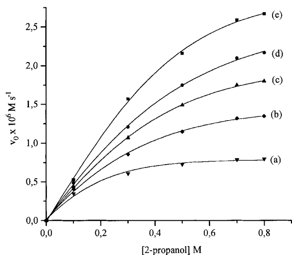
Figure 2. Dependence of v_0 on [2-propanol] at different [K_3Fe(CN)_6] . [Ru(VI)] = 4 \times 10^{-6} M , [NaOH] = 0.1 M , I = 0.5 M and T = 30^\circ C ; [K_3Fe(CN)_6] = (a) 0.2 \times 10^{-3} ; (b) 0.4 \times 10^{-3} ; (c) 0.8 \times 10^{-3} ; (d) 1.2 \times 10^{-3} ; (e) 1.6 \times 10^{-3} M
