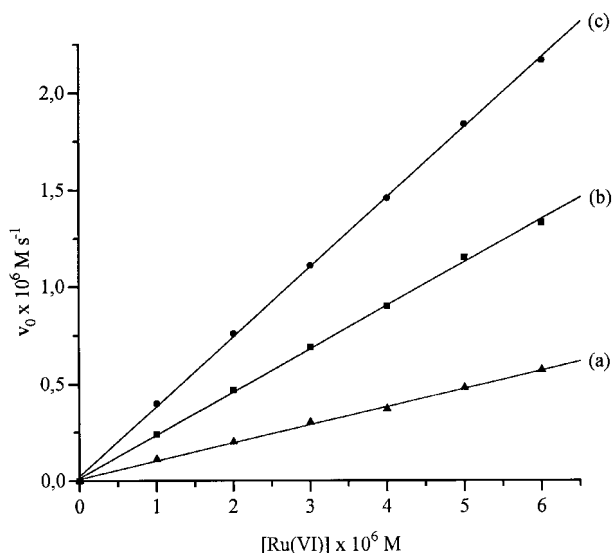
Figure 4. Plot of v_0 versus [\text{Ru(VI)}] . I = 0.5 \text{ M} and T = 30^\circ\text{C} ; (a) [\text{K}_3\text{Fe(CN)}_6] = 1.2 \times 10^{-3} \text{ M} , [\text{2-propanol}] = 0.2 \text{ M} , [\text{NaOH}] = 0.3 \text{ M} ; (b) [\text{K}_3\text{Fe(CN)}_6] = 0.8 \times 10^{-3} \text{ M} , [\text{2-propanol}] = 0.4 \text{ M} , [\text{NaOH}] = 0.2 \text{ M} ; (c) [\text{K}_3\text{Fe(CN)}_6] = 0.8 \times 10^{-3} \text{ M} , [\text{2-propanol}] = 0.5 \text{ M} , [\text{NaOH}] = 0.1 \text{ M}
